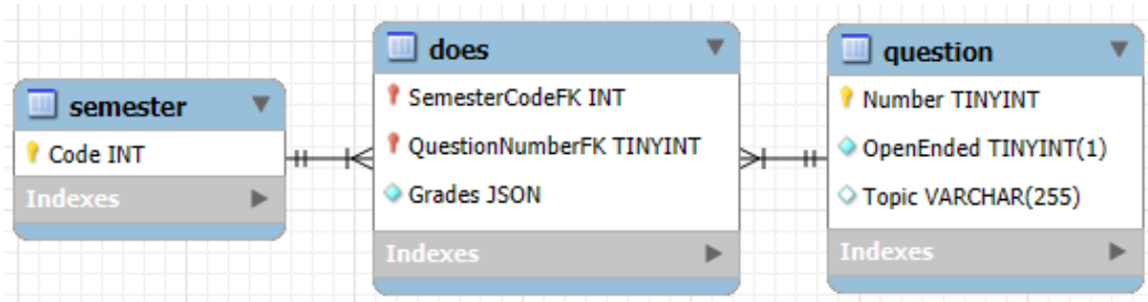
Figure 1: Entity-Relationship Data Model Concept. Generate by Reverse Engineering in MySQL Workbench.
